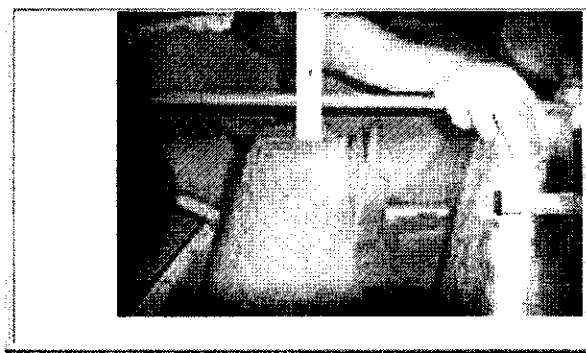
Figura 07 – Slump test
