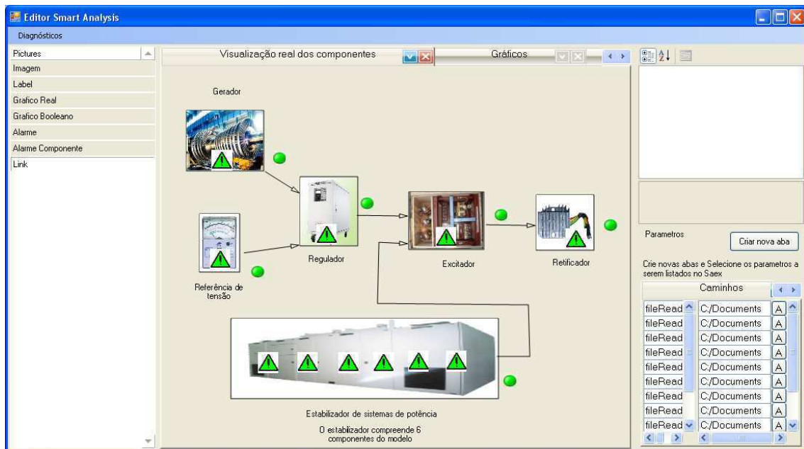
Figura 32: Tela principal do Auto-FDI Editor
