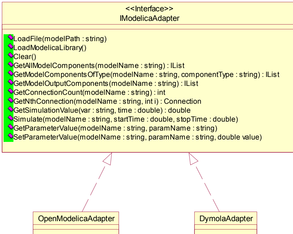
Figura 43: Diagrama de classes do pacote modelicacommunication
