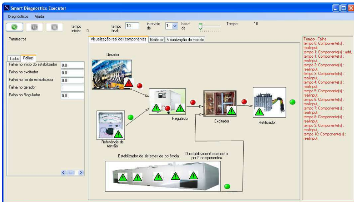
Figura 35: Tela principal do Auto-FDI Executor
